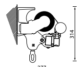
Australia R-Pitch Wall/Face Fix
