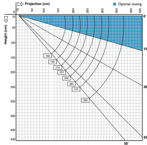
Australia with Semi-Cassette Front Bar Top Fix
