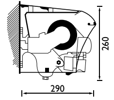
Australia with Hood Face Fix
