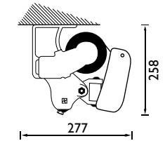
Australia with Semi-Cassette Front Bar Top Fix
